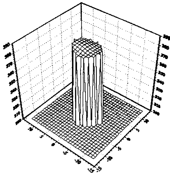
Fig. 3 Temperature distribution on a cross section of the test tube
