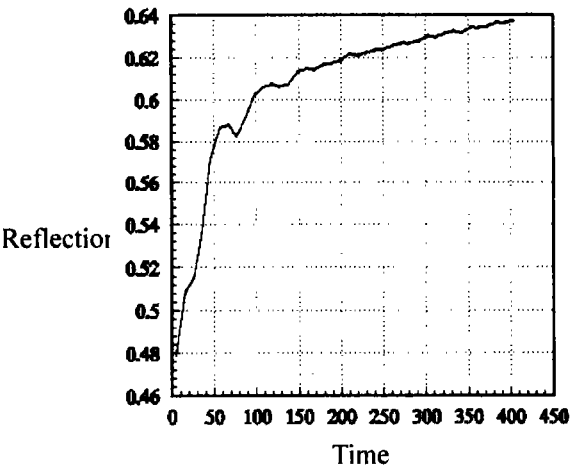
Fig. 2 Reflection variation due to dielectric constant change with chemical reaction
