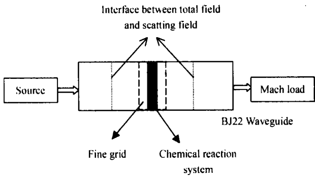
Fig. 1 Microwave chemical experimental system
